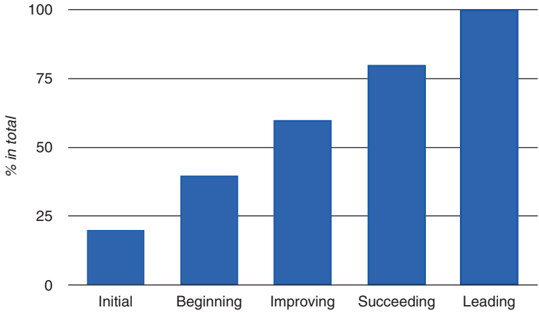
Fig. 8.3 Maturity levels
