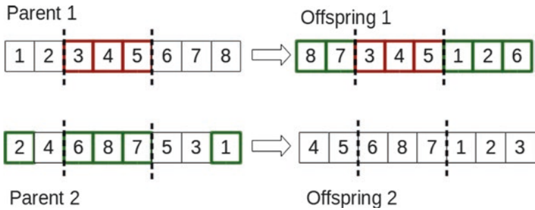
Fig. 4.5 Crossover operation
