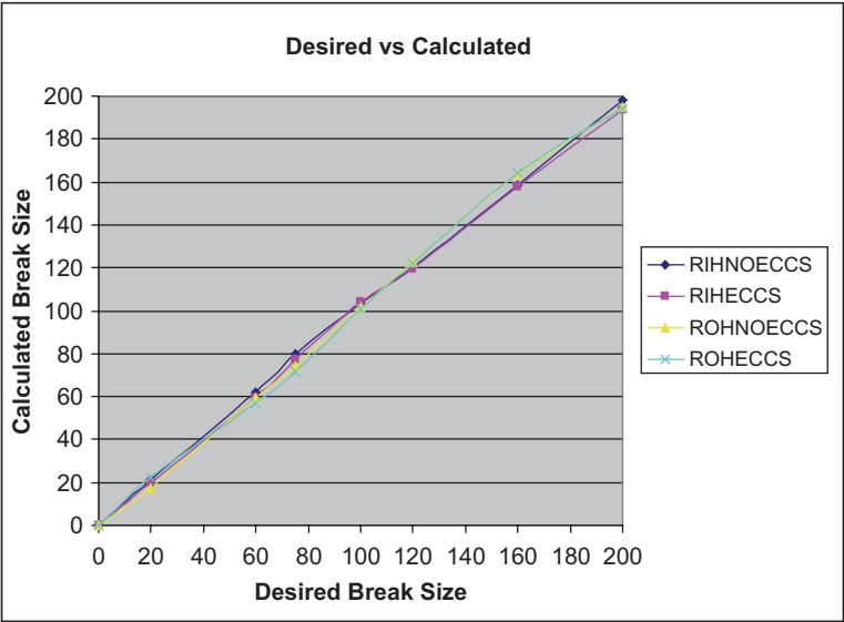
Fig. 17.4 Desired vs. calculated output of ANN
