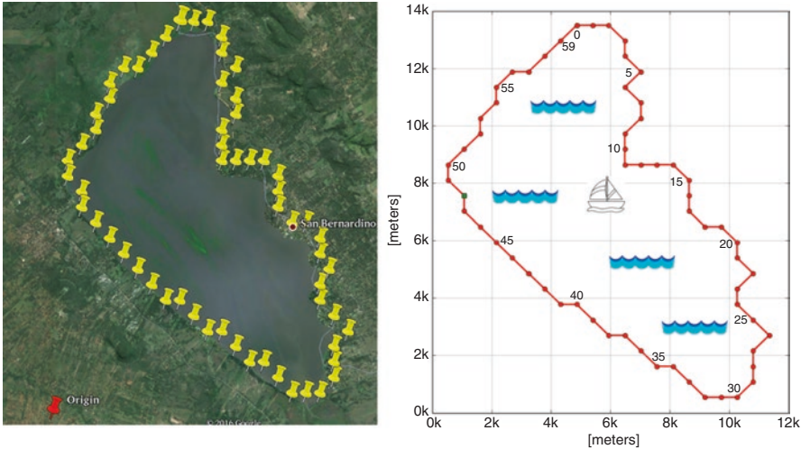
Fig. 4.3 (a) Beacon distribution and (b) numbering convention
