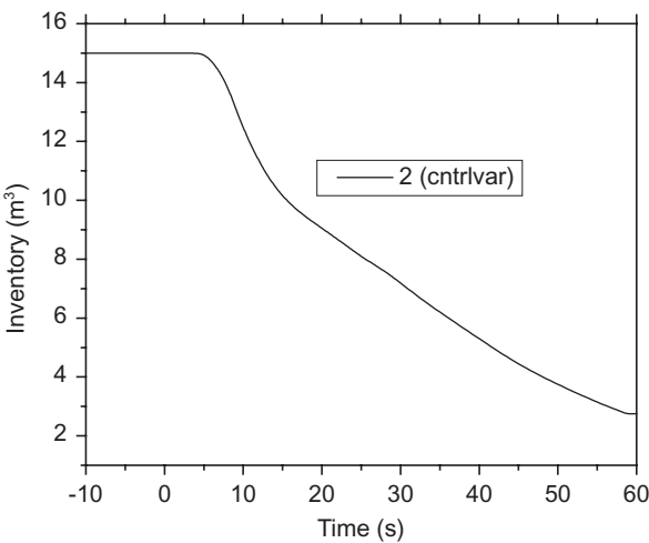
Fig. 17.3 D 2 O inventory in PHT system (m 3 )
