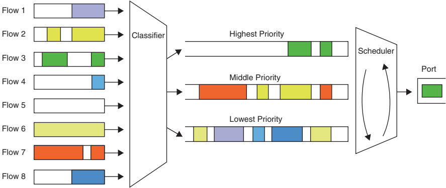
Fig. 9.13 Priority queuing mechanism
