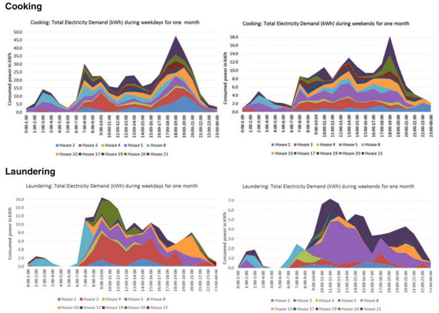
Fig. 4.2 Activity-based electricity demand during weekdays and weekends (Notes: Left panels show weekdays; Right panels show weekends; Demand was calculated for all 10 households for all activities shown, except washing which was calculated for five households)
