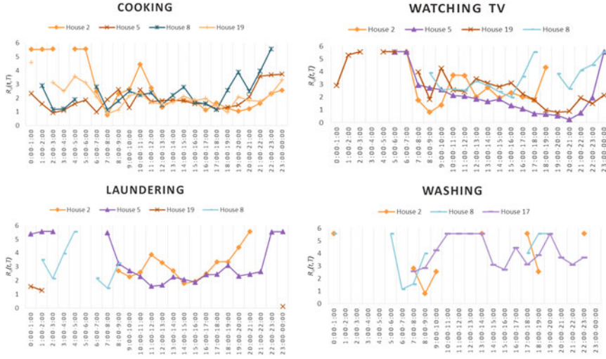
Fig. 4.6 Routine in the time profile of cooking, watching TV, laundering and washing in four houses during hourly timeslots over a one month period (Notes: Routine is measured using the routine metric, R_d(t, T) ; High values of R_d(t, T) indicate no routine during that timeslot (infrequent and/or inconsistent activities); Low values of R_d(t, T) indicate routine during that timeslot (frequent and/or consistent); Gap in values of R_d(t, T) indicates no activities during that timeslot)
