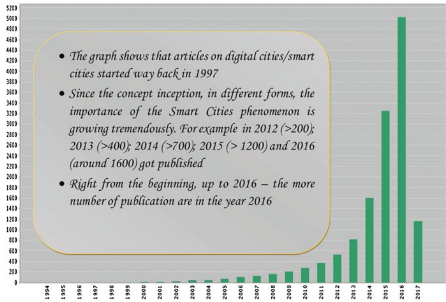
Graph 10.1 Articles published per year
