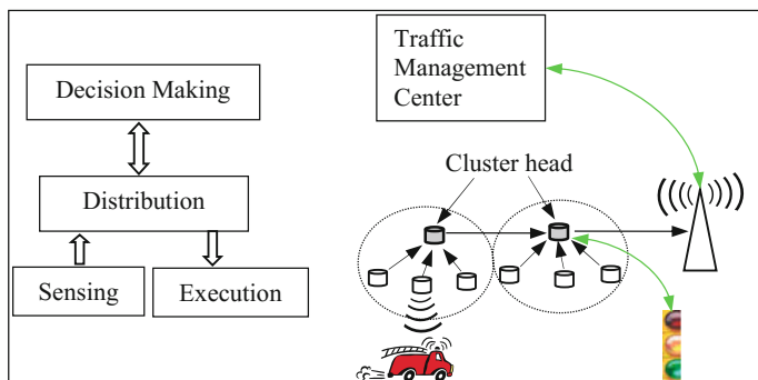
Fig. 5.2 Architecture of a WSN-based ITS
