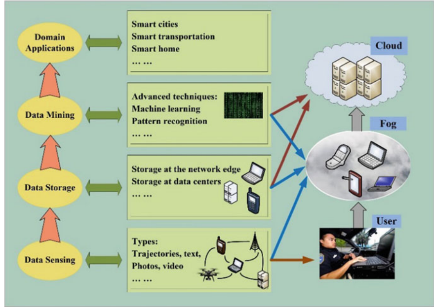
Fig. 7.1 A four-layer smart city architecture
