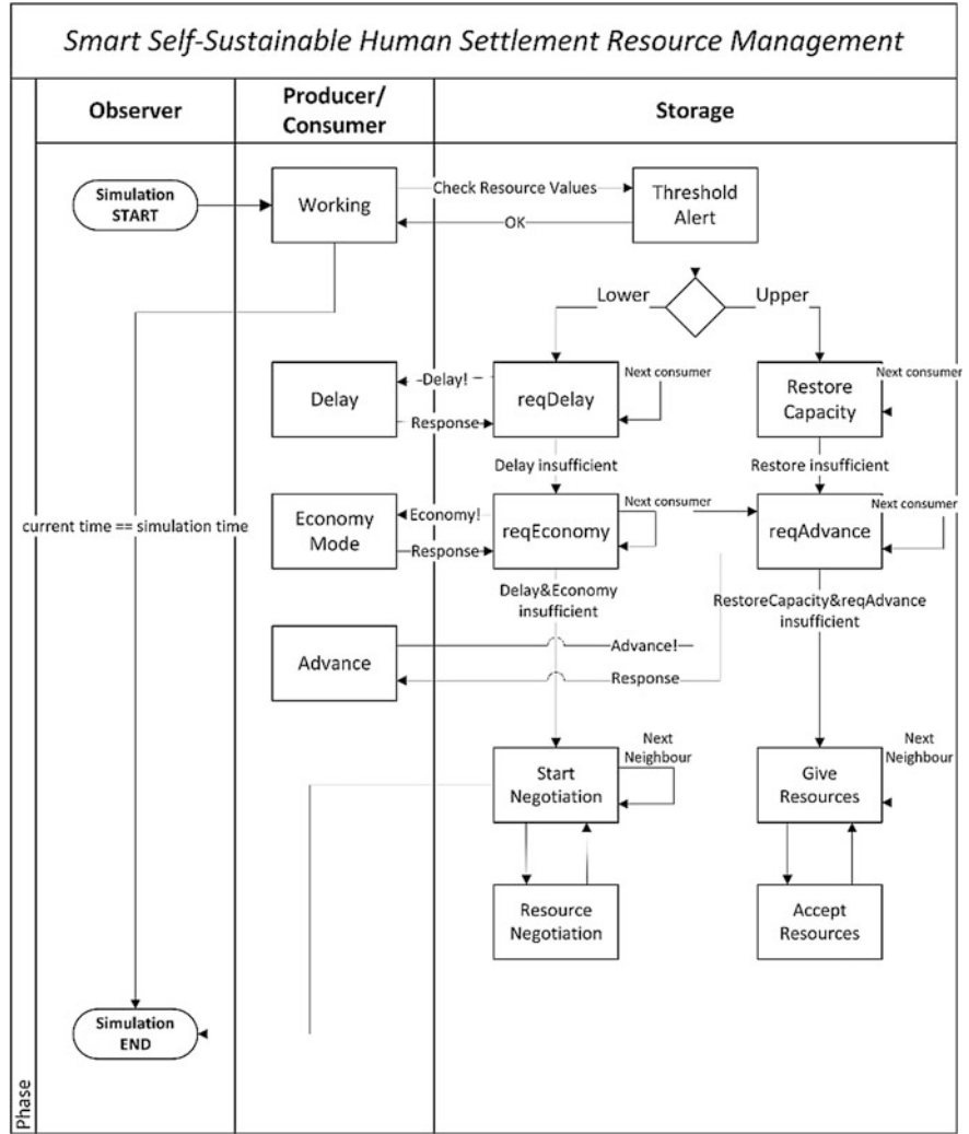
Fig. 1.4 The activity diagram of the SSSH framework (adopted from our previous work [26])
