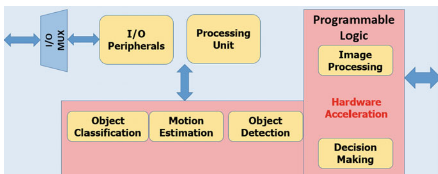
Fig. 9.6 Programmable SOC showing multiple processing units on a single chip
