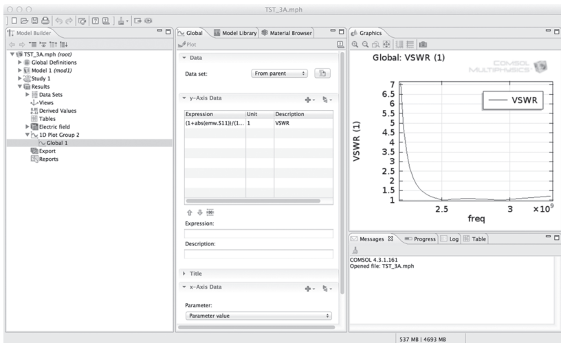
FIGURE 30. Three Stub Tuner Model TST_3A.mph on Desktop.
