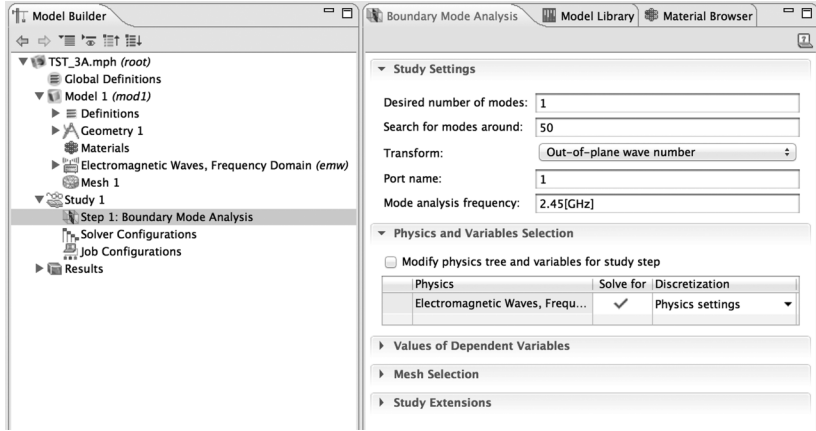
FIGURE 6. Boundary Mode Analysis Study Settings, Port 1.
