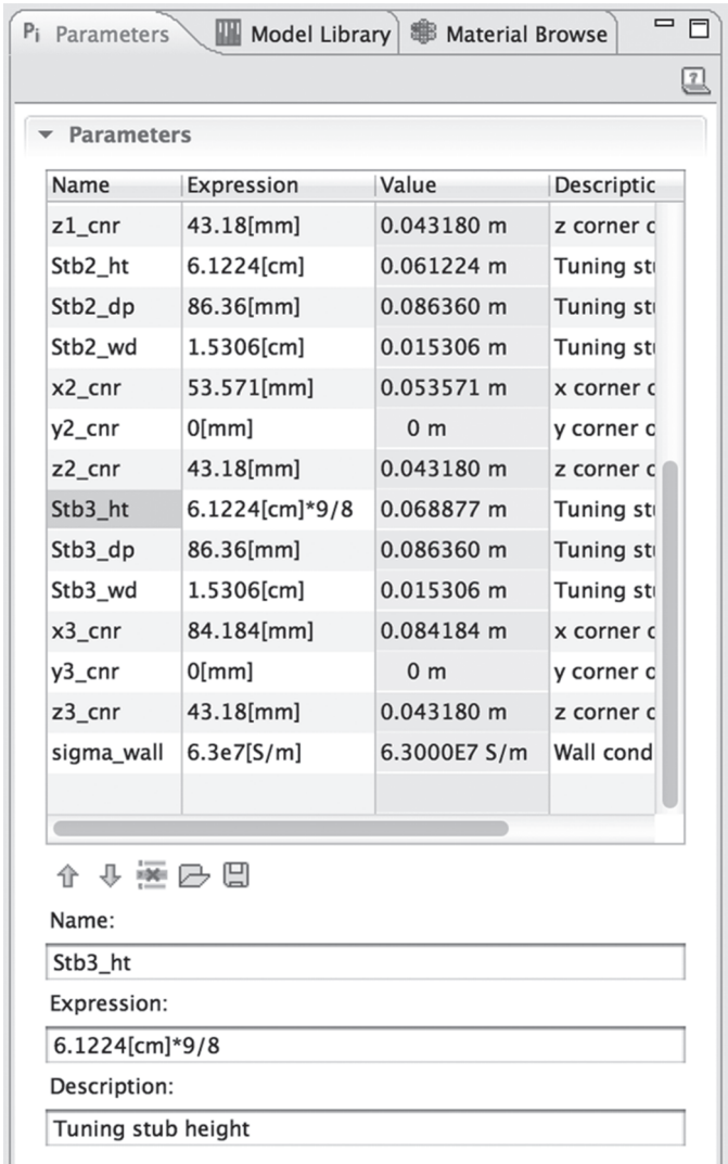
FIGURE 51. TST_3AM3.mph Parameters File Edit Window, Stb3_ht (Modified 3).
