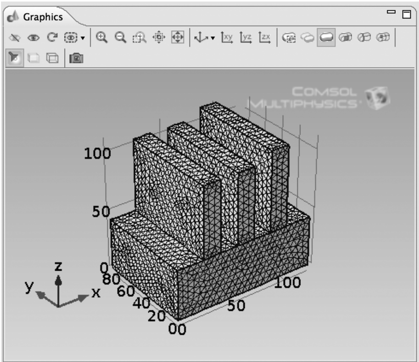
FIGURE 53. Three Stub Tuner Geometry (Modified 3) Meshed.
