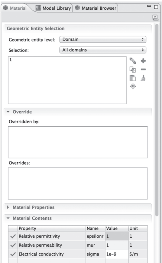
FIGURE 17. Materials Properties of Vacuum, as Configured.
