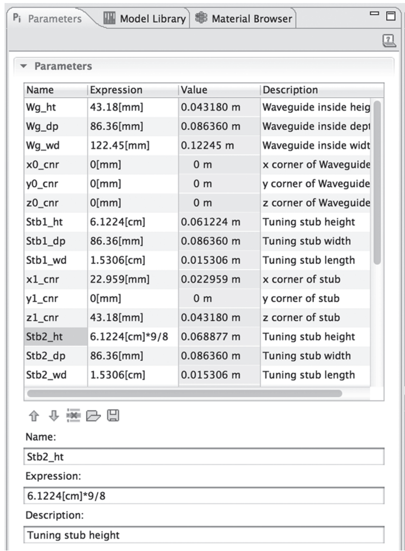
FIGURE 42. TST_3AM2.mph Parameters File Edit Window, Stb2_ht (Modified 2).
