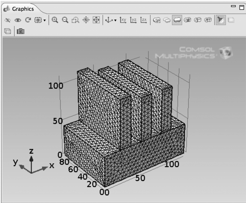
FIGURE 35. Three Stub Tuner Geometry (Modified) Meshed.
