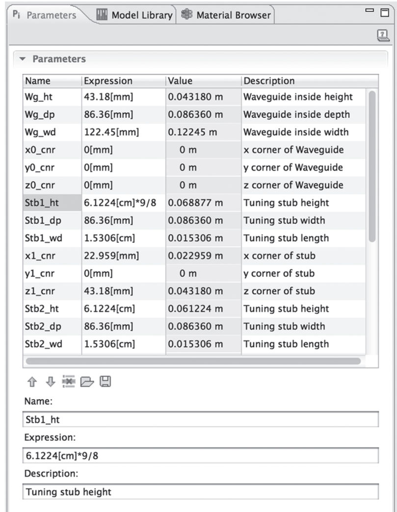
FIGURE 33. TST_3AM1.mph Parameters File Edit Window, Stb1_ht (Modified).
