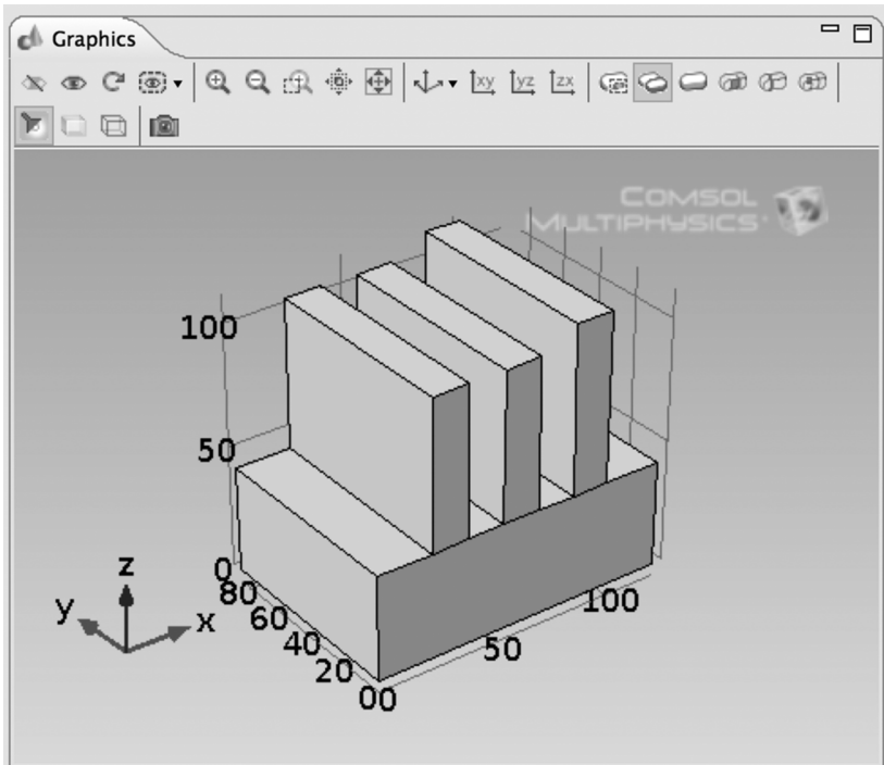
FIGURE 52. Three Stub Tuner Geometry (Modified 3).
