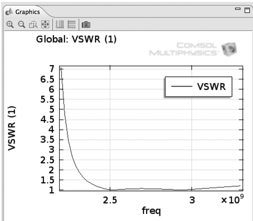
FIGURE 56. Three Stub Tuner VSWR.
