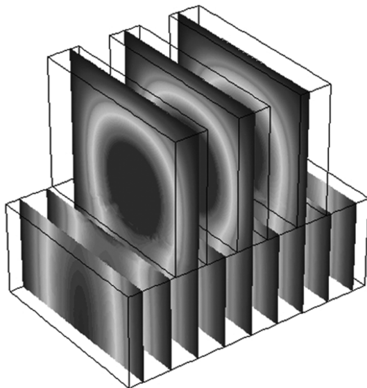
FIGURE 2. Three Stub Tuner Calculated Field-Distribution Solution.
