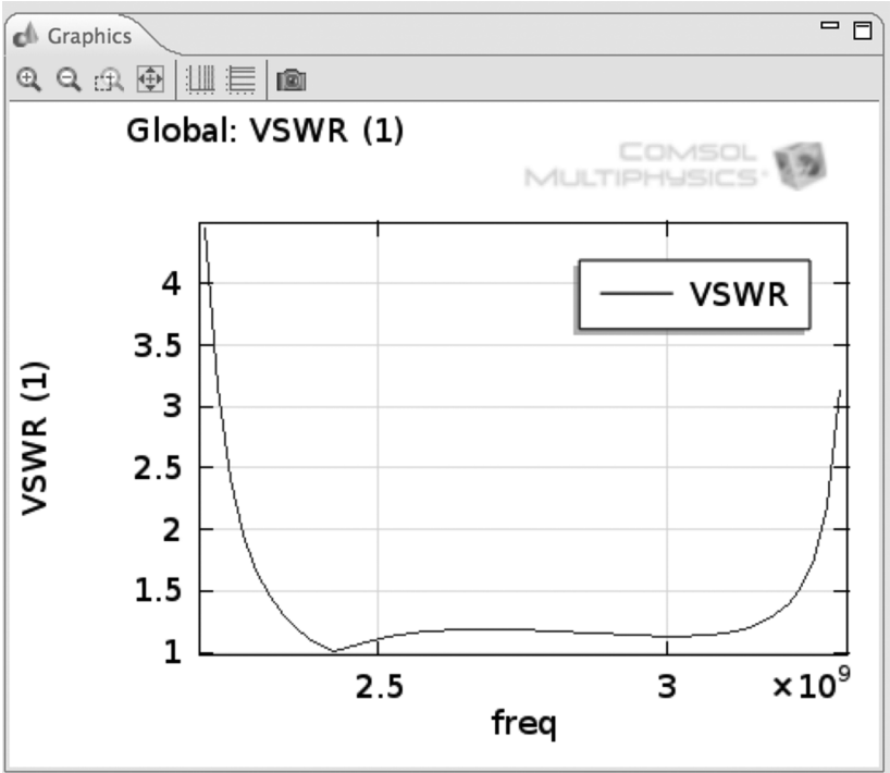
FIGURE 46. Three Stub Tuner (Modified 2) VSWR.
