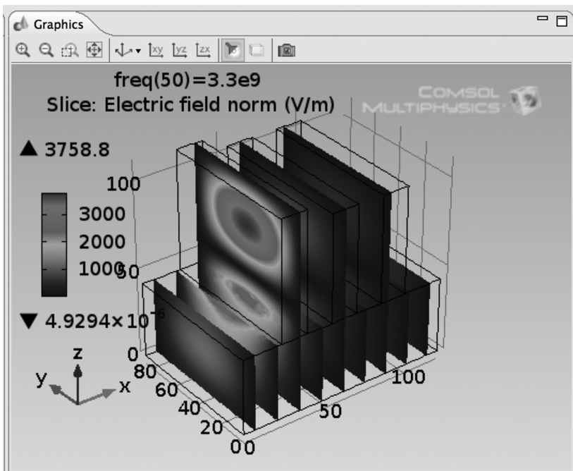
FIGURE 36. Three Stub Tuner (Modified) Electric Field Distribution.
