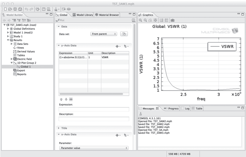
FIGURE 49. Three Stub Tuner Model TST_3AM3.mph on Desktop.
