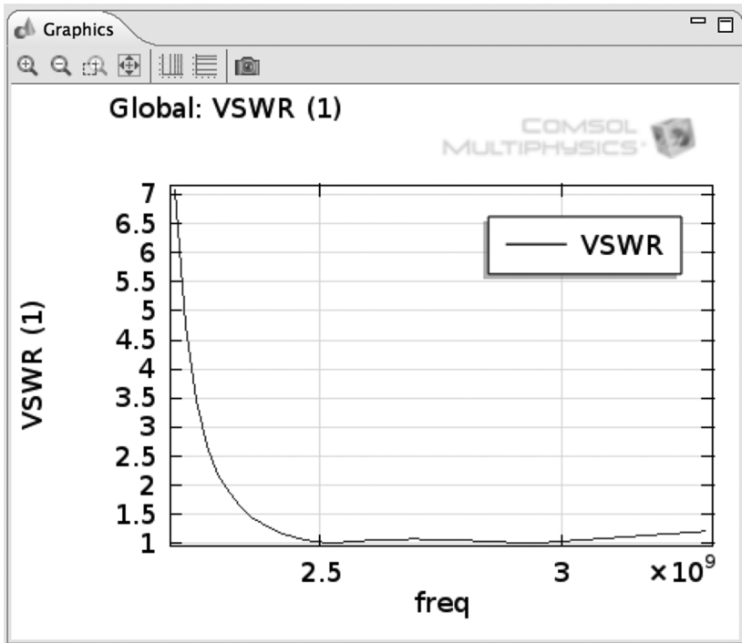
FIGURE 47. Three Stub Tuner VSWR.
