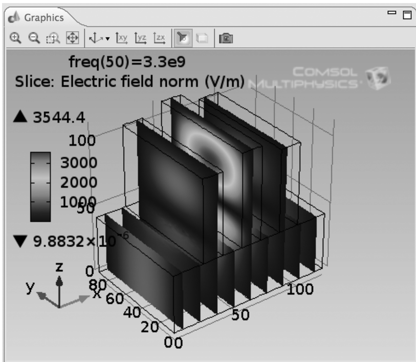
FIGURE 45. Three Stub Tuner (Modified 2) Electric Field Distribution.
