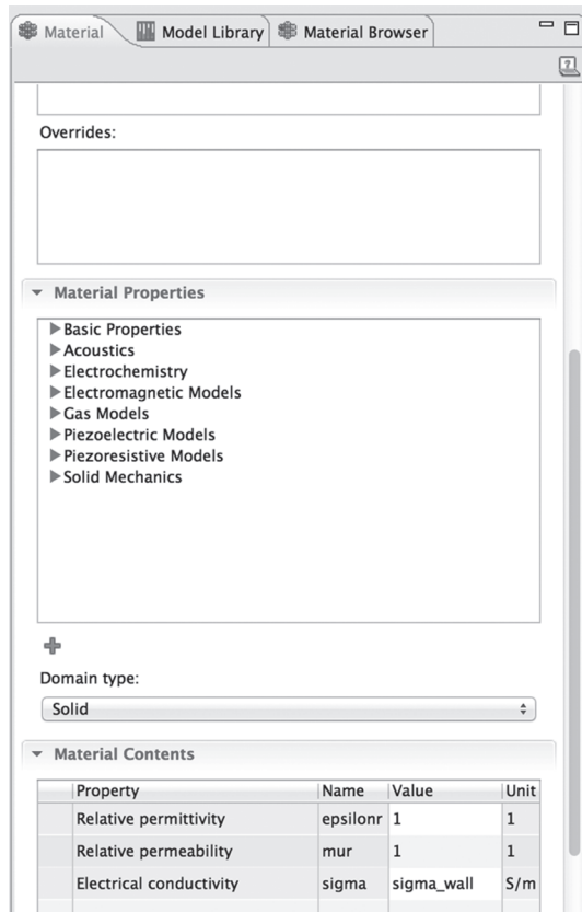
FIGURE 19. Lossy Wall Properties, as Configured.
