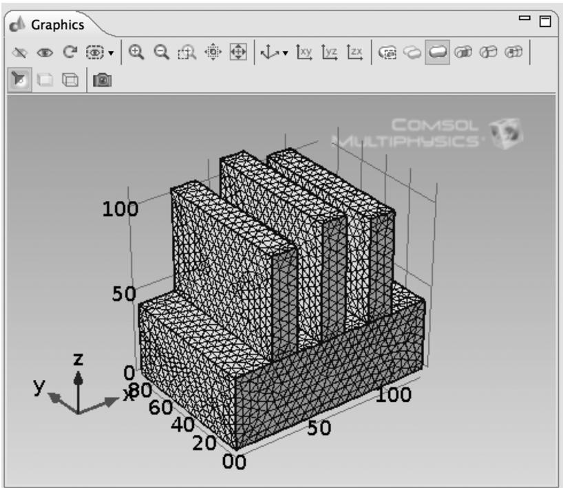
FIGURE 44. Three Stub Tuner Geometry (Modified 2) Meshed.
