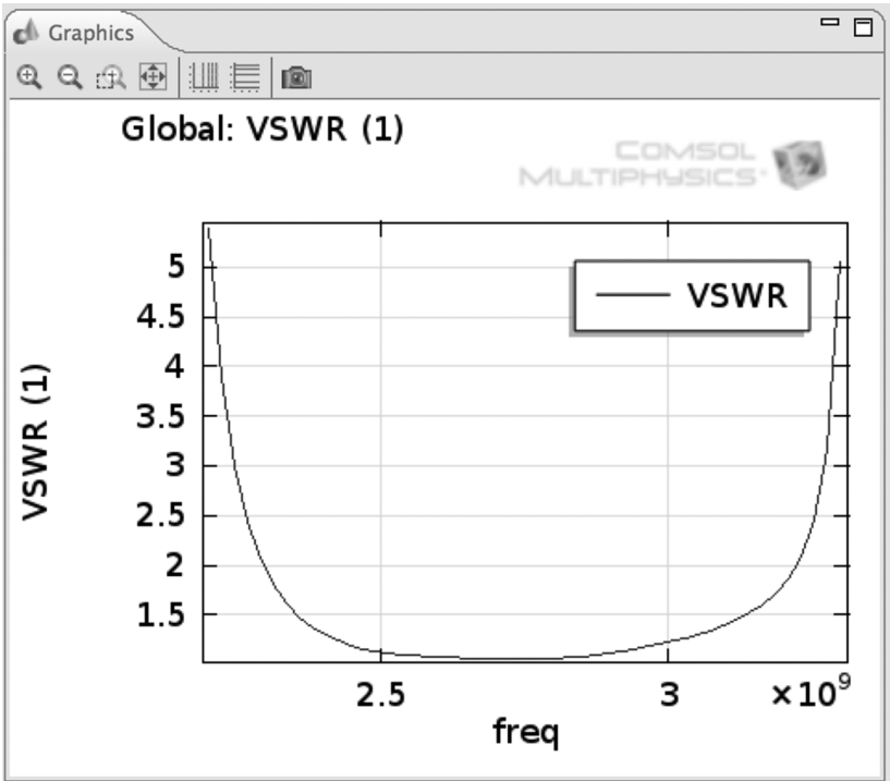
FIGURE 55. Three Stub Tuner (Modified 3) VSWR.
