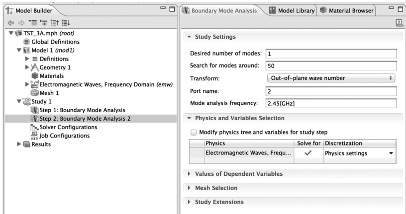
FIGURE 7. Boundary Mode Analysis Study Settings, Port 2.
