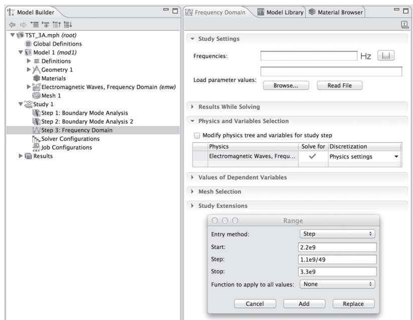
FIGURE 9. Frequency Domain, Step 3 Settings, as Configured.
