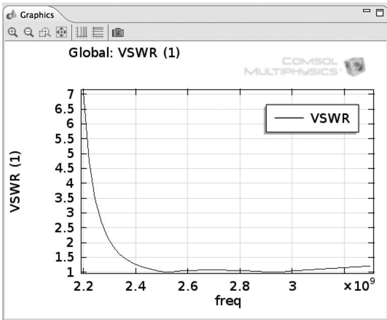
FIGURE 38. Three Stub Tuner VSWR.
