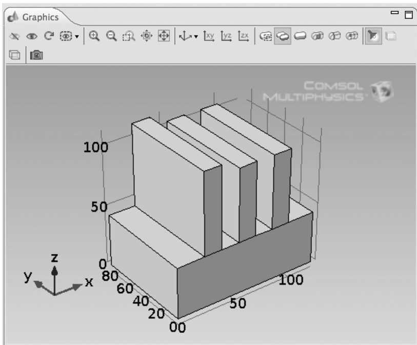
FIGURE 34. Three Stub Tuner Geometry (Modified).
