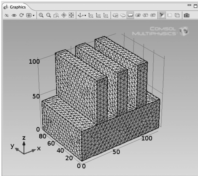
FIGURE 25. Meshed Model.
