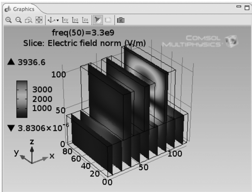
FIGURE 54. Three Stub Tuner (Modified 3) Electric Field Distribution.
