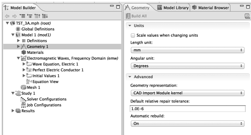
FIGURE 4. Initial Three Stub Tuner Model Builder Tree.
