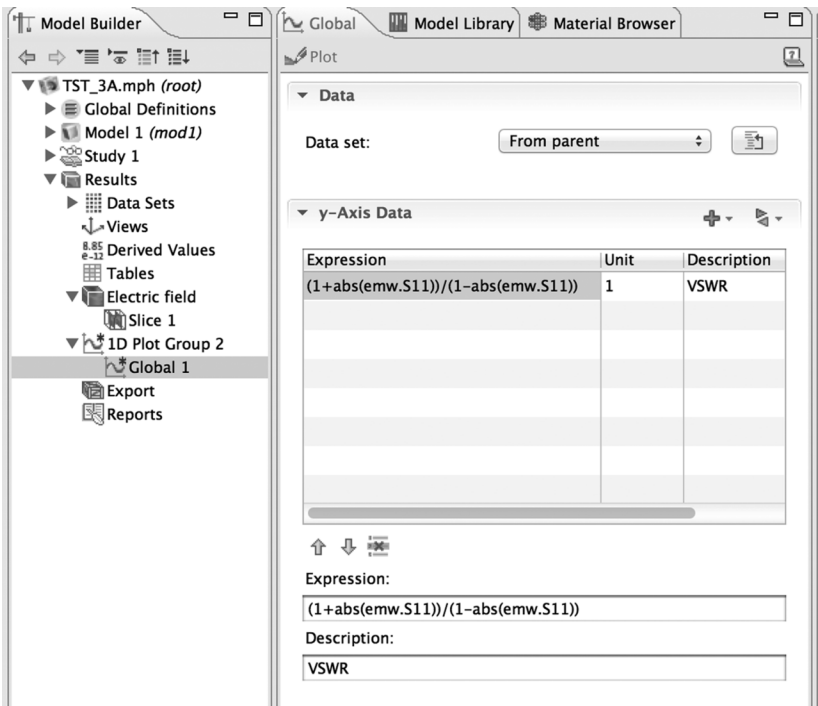
FIGURE 28. VSWR Calculation Settings.
