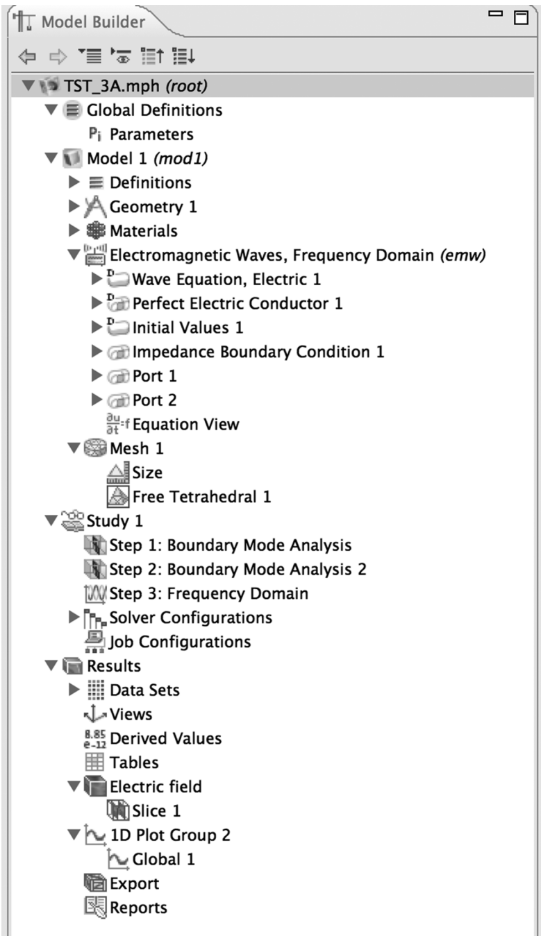
FIGURE 3. The Completed Three Stub Tuner Model Builder Tree.
