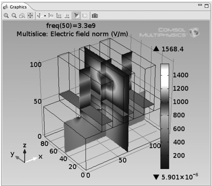
FIGURE 26. Calculated Three Stub Tuner Electric Field, Default Settings.
