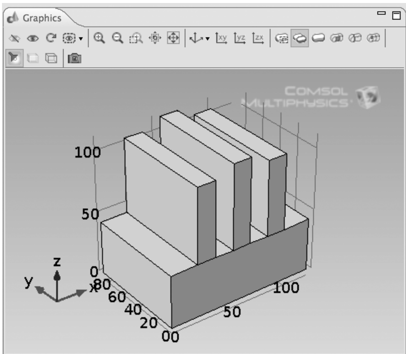
FIGURE 43. Three Stub Tuner Geometry (Modified 2).
