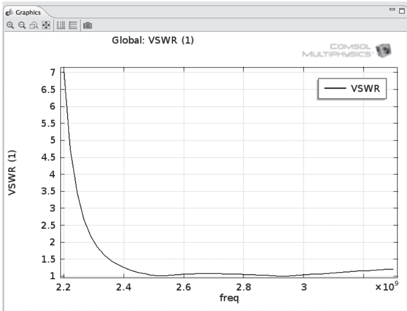
FIGURE 29. Three Stub Tuner Model VSWR Plot.
