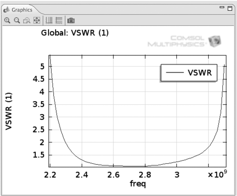
FIGURE 37. Three Stub Tuner (Modified) VSWR.
