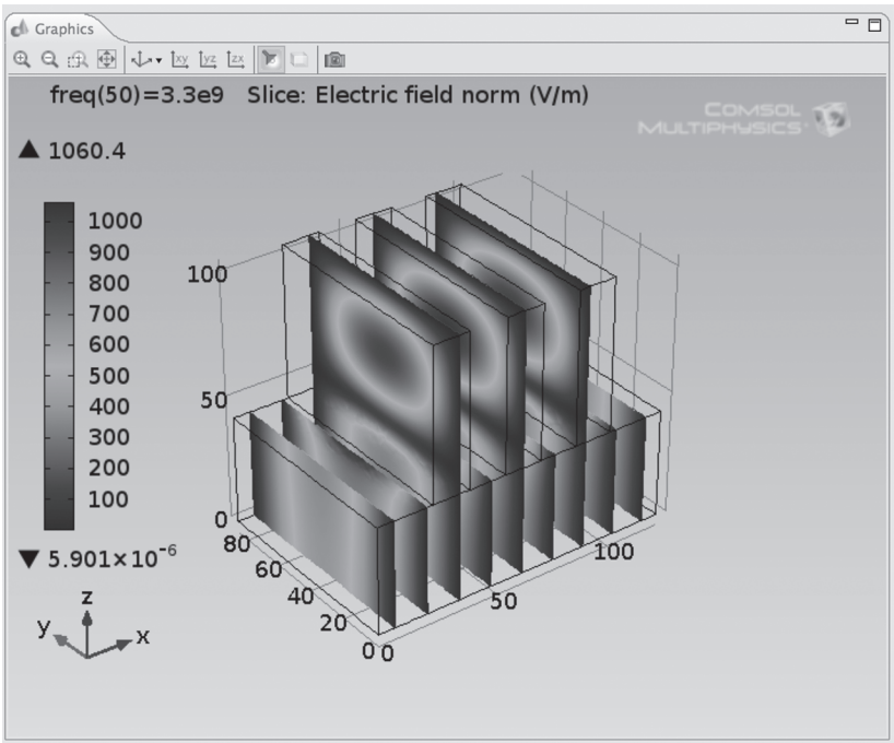
FIGURE 27. Calculated Three Stub Tuner Electric Field, Revised Settings.
