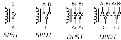
Relays
